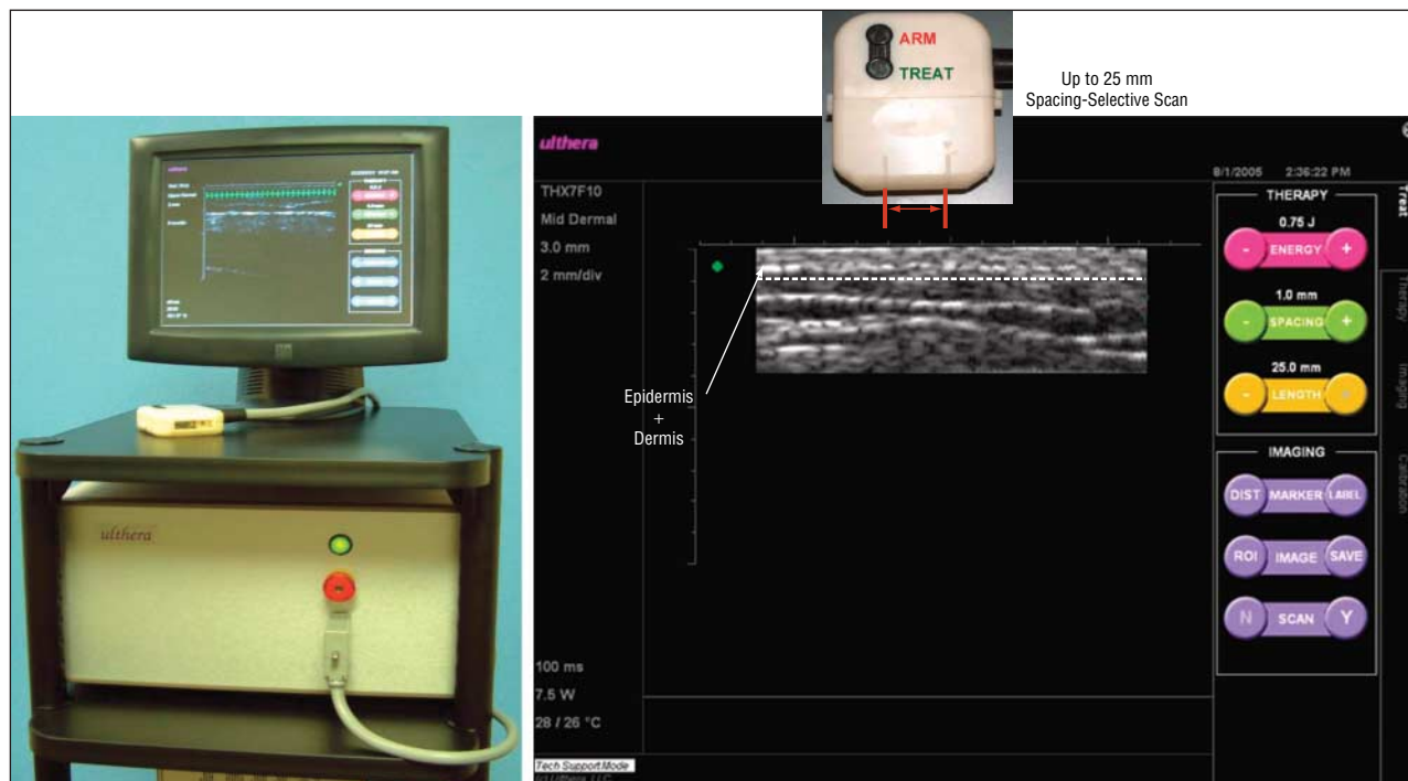
Figure 1. Intense ultrasound system. Imaging and treatment are possible with the same handpiece.
